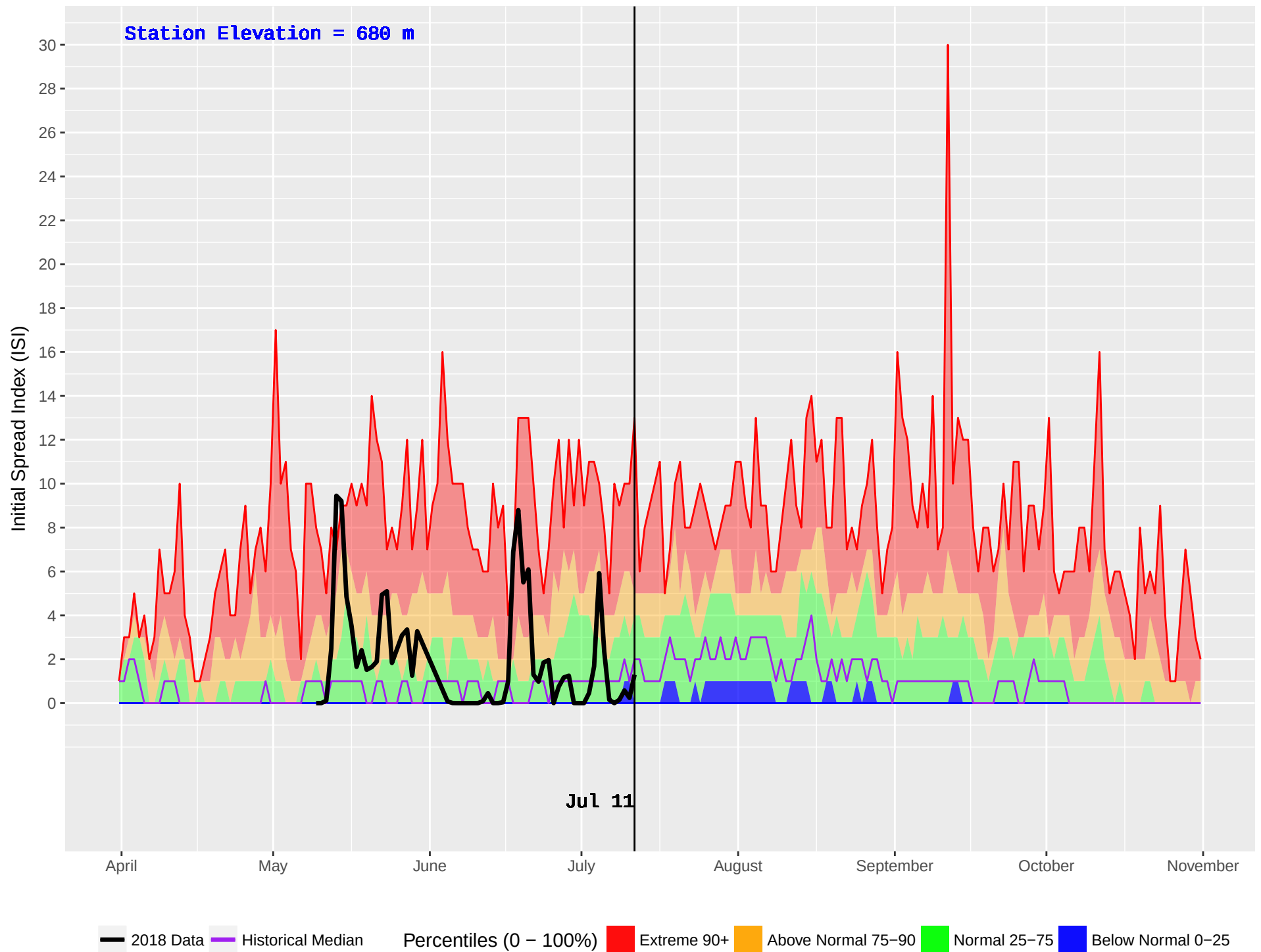
SUMMIT (11) : Historical (1985–2016) and Current (2018) Noon Initial Spread Index (ISI)
